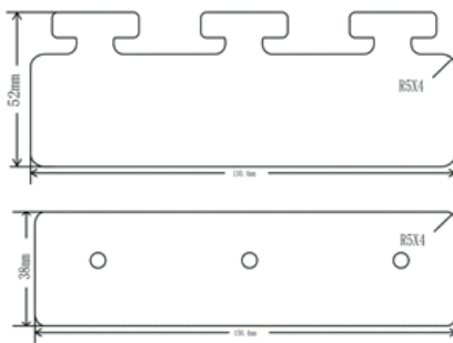
Holders for 200mm width PVC strip
