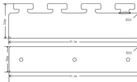
Holders for 300mm width PVC strip
