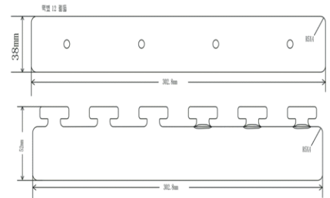
Holders for 400mm width PVC strip
